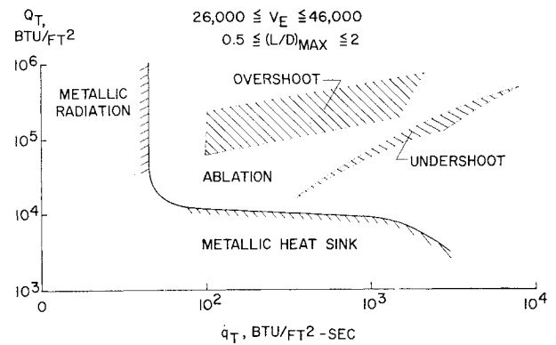
Fig. 12 Total stagnation-point heating in relation to heat protection. Entry at (L/D)_{max} , mode U .
