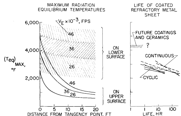
Fig. 13 Surface temperatures and material capability.
