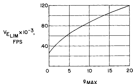
Fig. 3 Effect of deceleration on limiting entry velocity.
