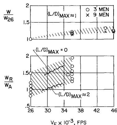
Fig. 16 Effect of entry velocity on entry vehicle weight; literature survey.
