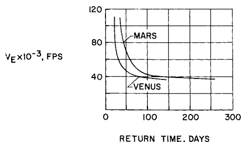
Fig. 2 Relation of transit time from Mars and Venus to minimum earth entry velocity.
